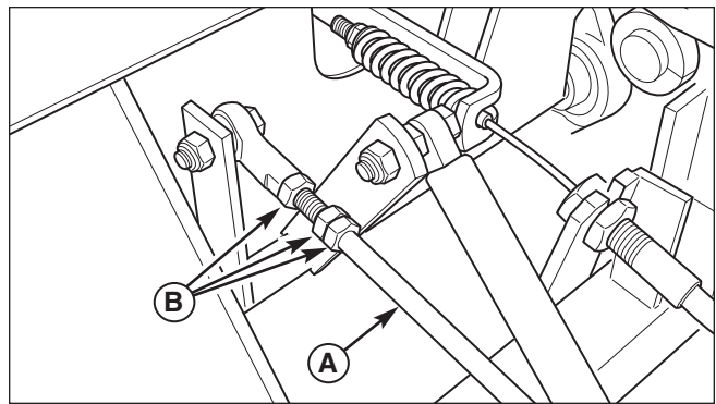
Figure 31. Neutral Adjustment (RH side shown) A. Adjustment Linkage Rod B. Nuts
