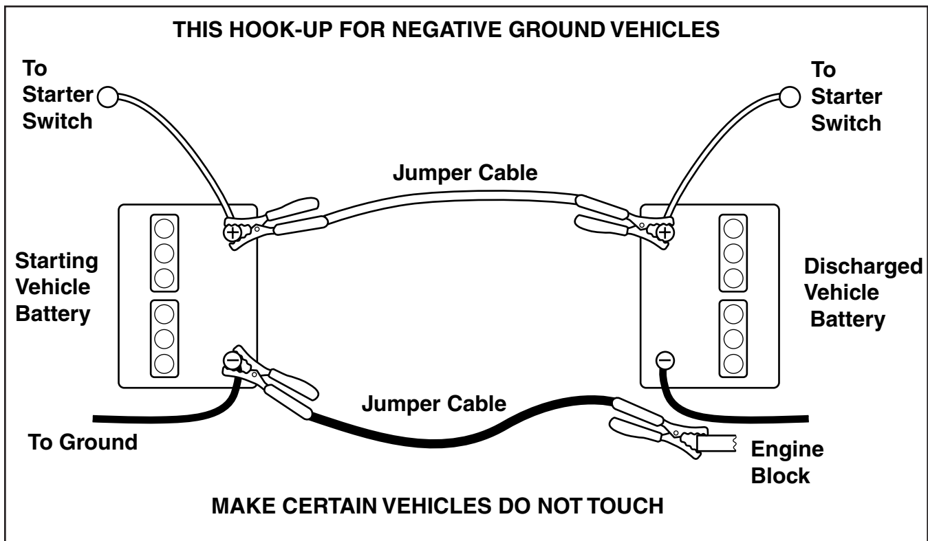
Figure 46. Jump Starting
