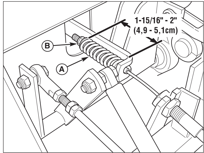
Figure 33. Parking Brake Adjustment
