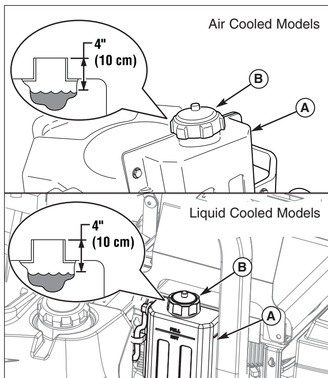
Figure 16. Checking Hydraulic Oil Level A. Hydraulic Oil Reservoir B. Reservoir Cap
