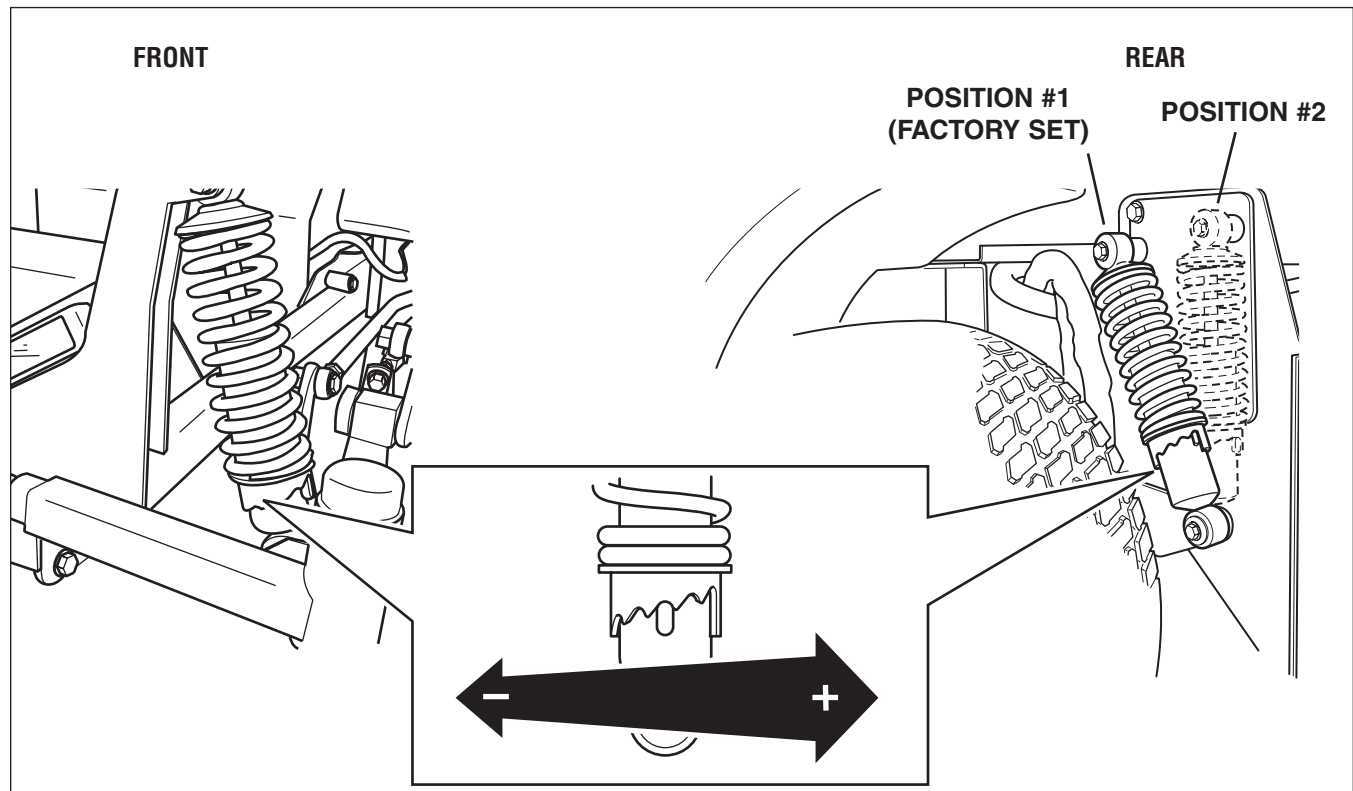
Figure 34. Suspension Adjustment
