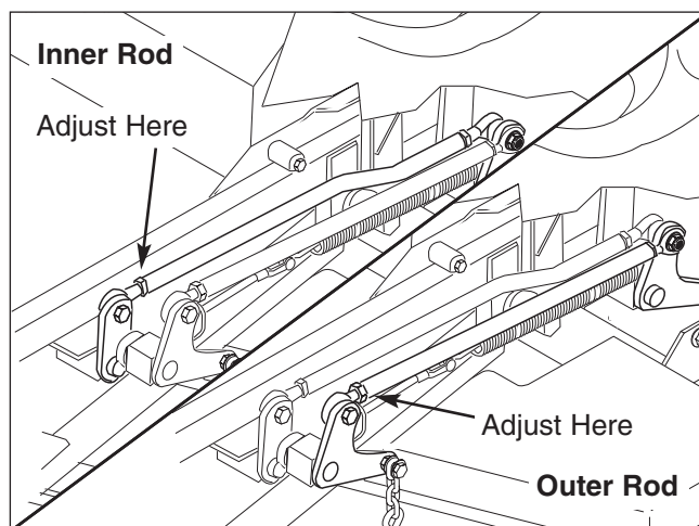
Figure 39. Adjust the Inner & Outer Lift Rods
